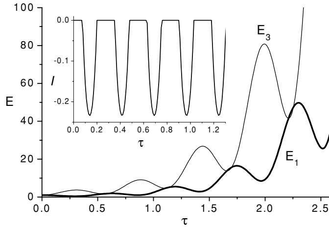
Figure 1. The normalized energies E_k(\tau) \equiv \mathcal{E}_k(\tau)/\mathcal{E}_k(0) of the first and third modes in a cubic cavity with resonantly oscillating boundary ( \gamma = 50/3 ) versus the 'slow time' \tau , for initial highly squeezed thermal states with \vartheta_1 = 3\vartheta_3 = 100 , r_1 = r_3 = 2.5 , and \chi_1 = \chi_3 = 0 . In the insertion: the inverse negativity coefficient \mathcal{I} (16) between the first and third modes under the same initial conditions.
